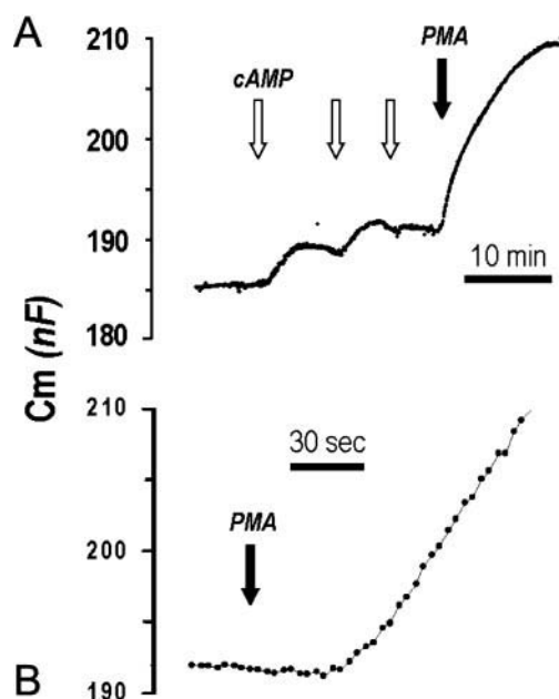
FIGURE 7 Measuring small and fast C_m changes in Xenopus oocytes using paired voltage ramps. (A) Effect of cAMP on C_m in native Xenopus oocyte. White arrows indicate 100-s incubations in 100 \mu M 8-Br-cAMP, and black arrow indicates 100-s incubation in 1.0 \mu M phorbol-12-myristate 13-acetate (PMA). The findings suggest that PKA and PKC regulate two distinct pools of potential exocytotic vesicles. (B) Effect of PMA on C_m in native Xenopus oocyte. Arrow indicates 100-s incubation in 1.0 \mu M PMA. Assuming diameters of the exocytotic vesicles of 180 nm, corresponding to 0.8 fF, the observed exocytosis rate implies \sim 375,000 fusion events per second. Here, voltage ramps with a downward slope of 1 V/s were used (cf. Fig. 3 A).
